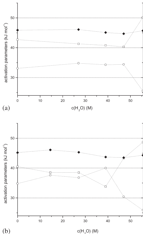
Figure 8. Activation parameters for the reaction of 1 with (a) 2a and (b) 2b in water–1-propanol mixtures at 25 °C: \Delta^\ddagger G^\circ - 30 (◆); \Delta^\ddagger H^\circ (□); -T\Delta^\ddagger S^\circ
