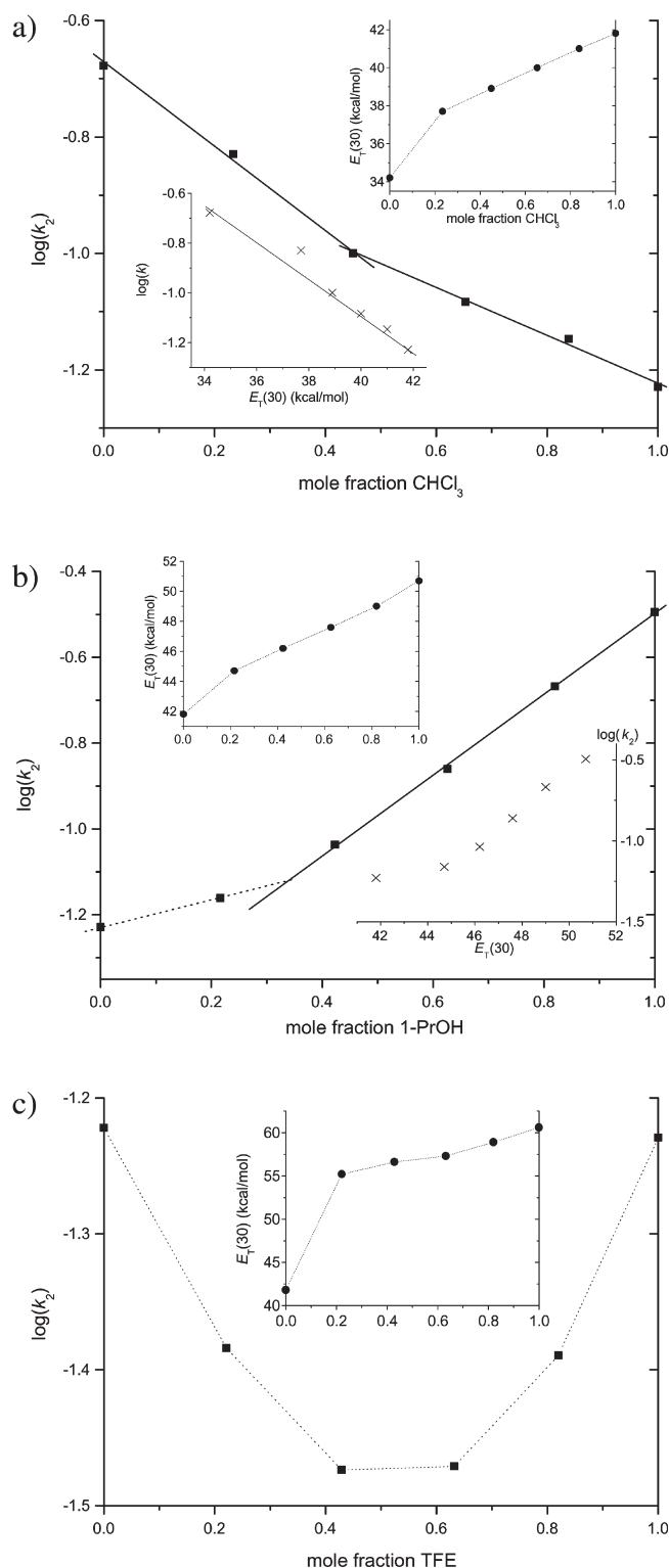
Figure 4. Logarithms of the bimolecular rate constants ( \text{M}^{-1} \text{s}^{-1} ) of the reaction of 2a with 1 in mixtures of chloroform with (a) \text{CCl}_4 , (b) 1-propanol and (c) TFE at 25 °C. (In all cases, the plots hardly differ when converted to a molar scale, as in all cases the molar volumes of the solvents are similar and the extent of non-ideal mixing limited.) The insets show the corresponding E_T(30) values and \log k_2 vs E_T(30)
