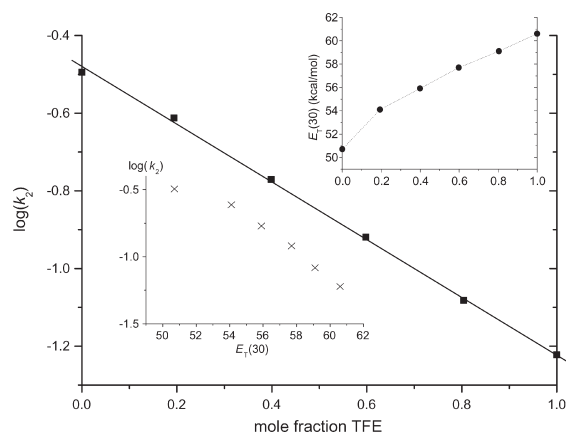
Figure 5. Logarithms of the bimolecular rate constants ( \text{M}^{-1} \text{s}^{-1} ) of the reaction of 2a with 1 in mixtures of 1-propanol with TFE at 25 °C. The insets show the corresponding E_T(30) values and \log k_2 vs E_T(30)
